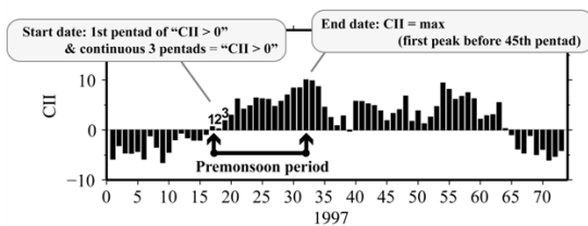
Fig. 4. Method of determination for the start date and the end date of the premonsoon period using CII. The horizontal axis means the pentad numbers. The vertical axis indicates the CII values.
